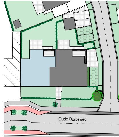
Inplantingsplan
